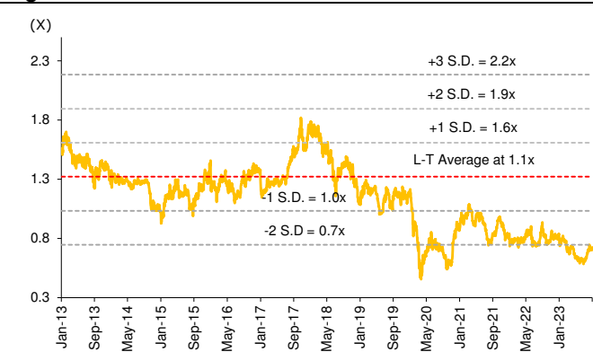
Figure 14: TOP P/BV Band
