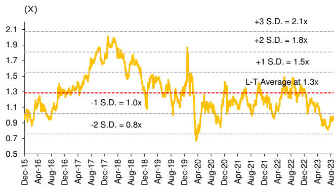
Figure 12: SPRC P/BV Band
