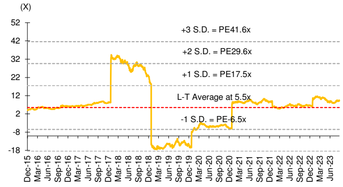
Figure 13: SPRC P/E Band
