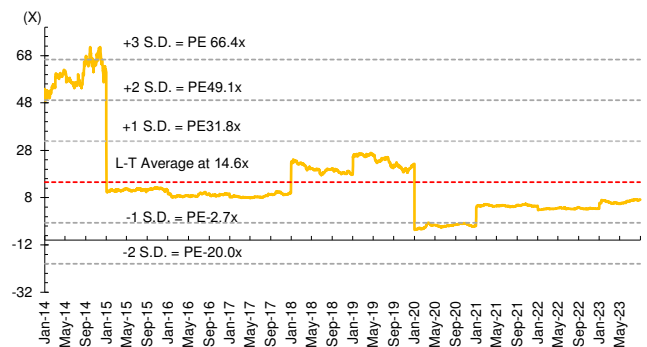
Figure 11: BCP P/E Band
