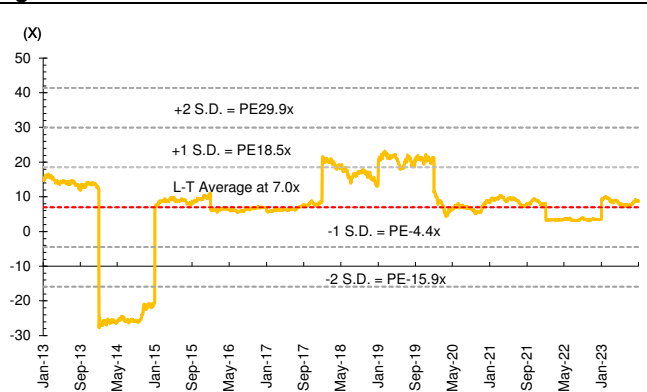
Figure 15: TOP P/E Band
