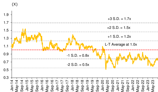
Figure 10: BCP P/BV Band
