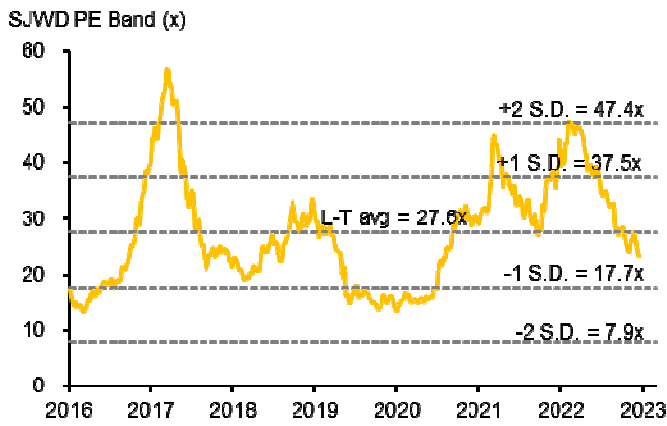
Figure 1: P/E band
