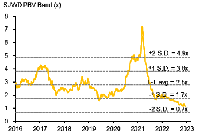
Figure 2: P/BV band
