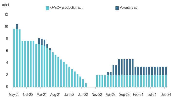
Fig 2: OPEC+ production/voluntary cut trend
