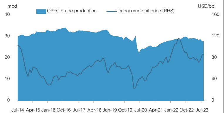
Fig 3: OPEC crude production vs Dubai crude oil price
