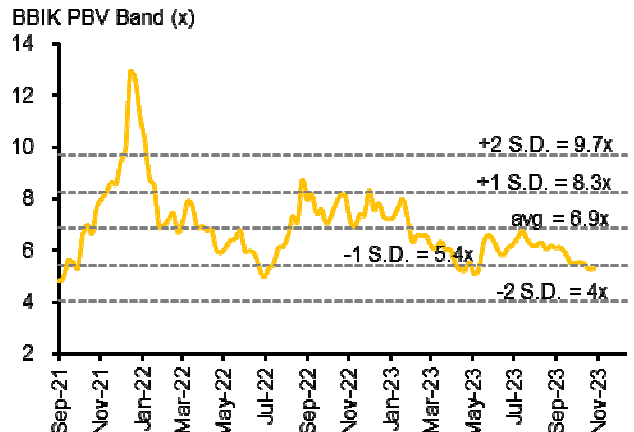
Figure 4: P/BV band
