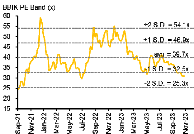
Figure 3: P/E band
