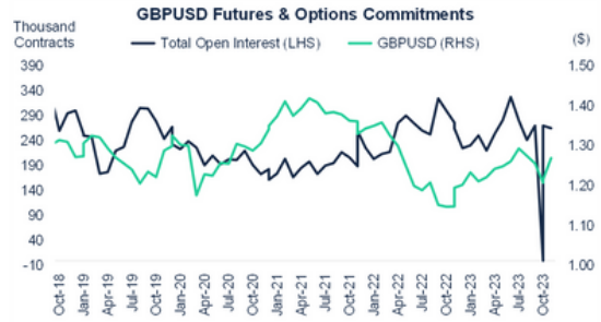
Source: Bloomberg,CFTC
