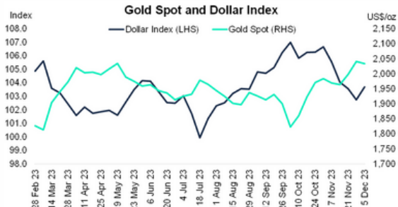
Source: Bloomberg
