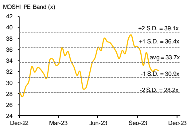
Figure 2: P/E band
