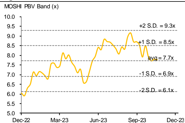
Figure 3: P/BV band
