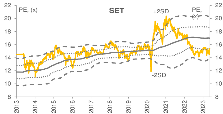
Figure 3: SET Index is trading at undemanding PE valuation (-1SD of mean)
