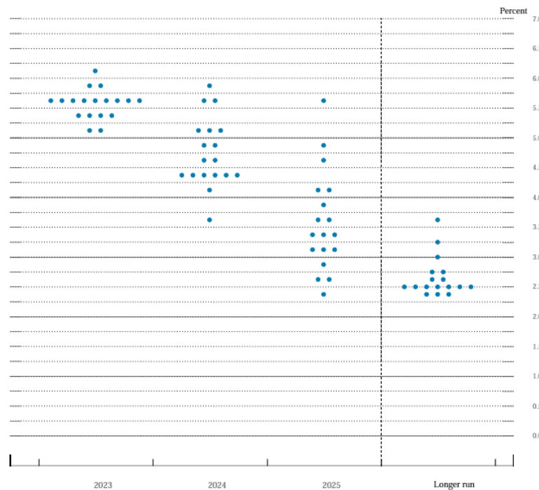
Figure 2: June dot plots
