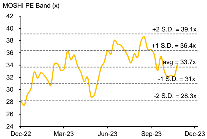
Figure 1: P/E band
