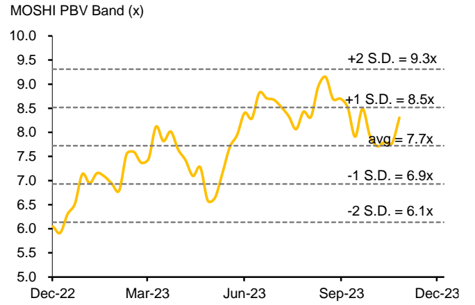
Figure 2: P/BV band
