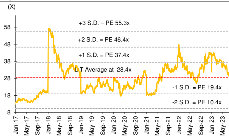
Figure 1: P/E band
