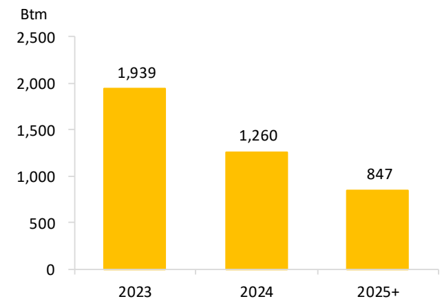
Figure 17: GABLE's backlog
