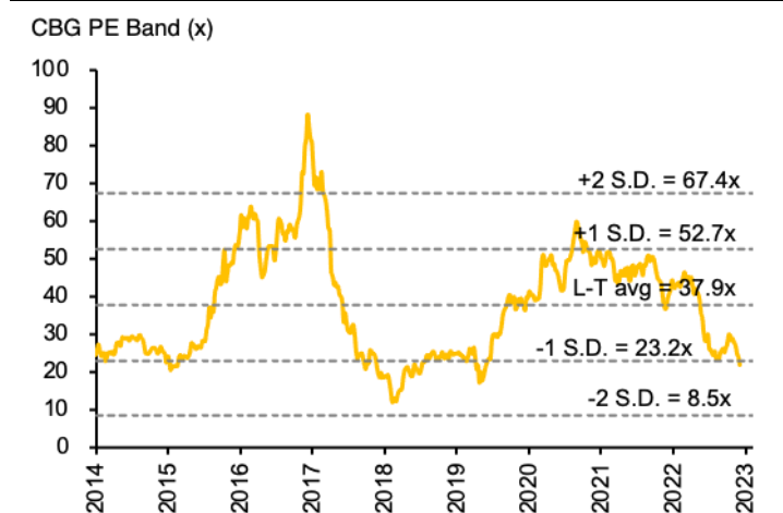
Figure 3: P/E band
