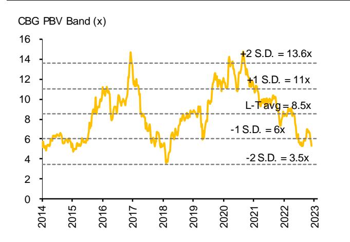
Figure 4: P/BV band
