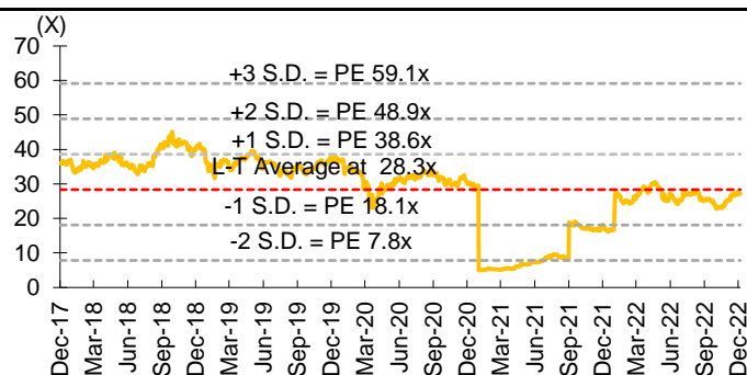
Fig 7: P/E band
