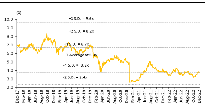
Fig 8: P/BV band
