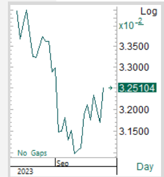
TOP/SET
