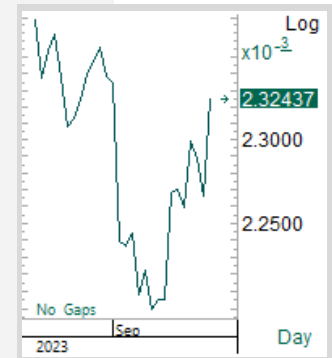
TOP/ENERG
