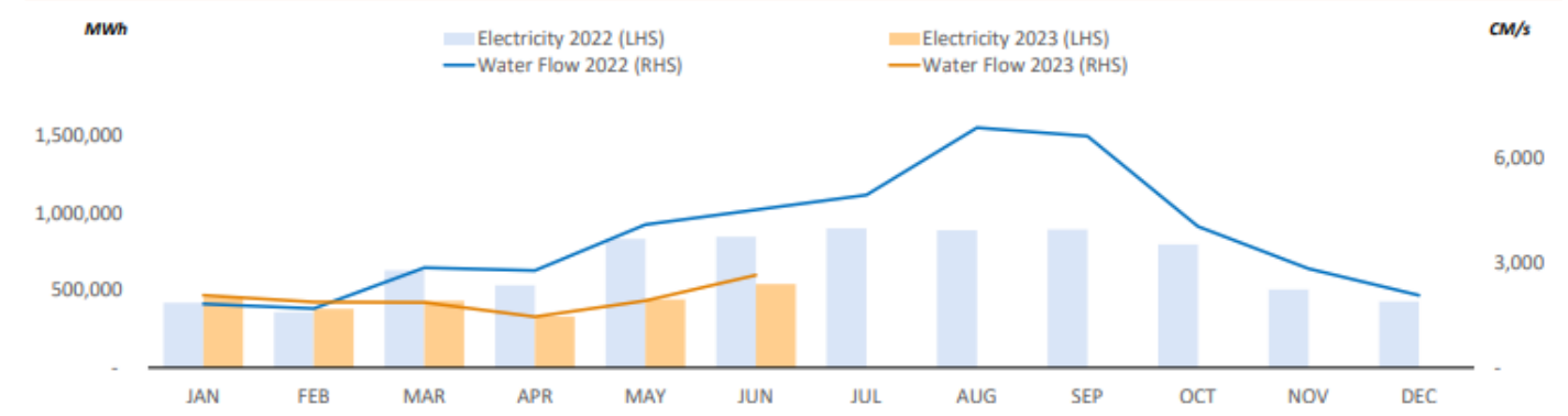
Figure 7: Xayaburi hydro power plant (XPCL) operating statistics
