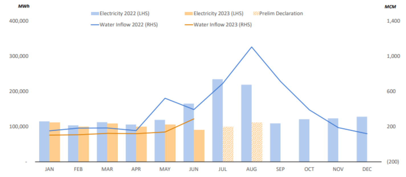
Figure 6: Nam Ngum 2 hydro power plant (NN2) operating statistics
