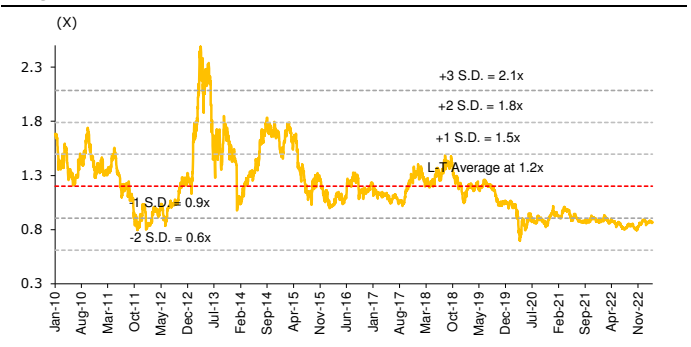
Figure 3: PBV band
