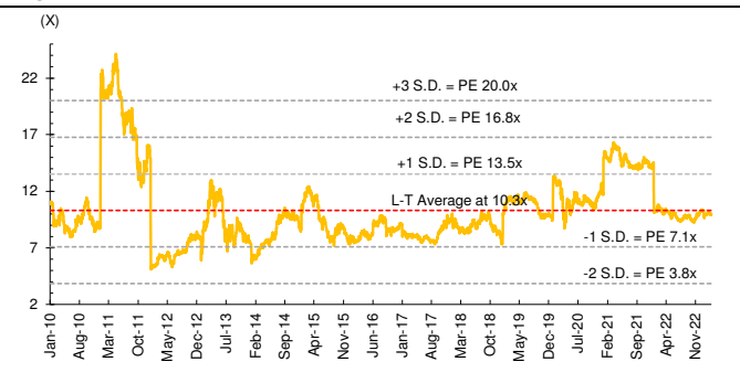
Figure 2: PER band
