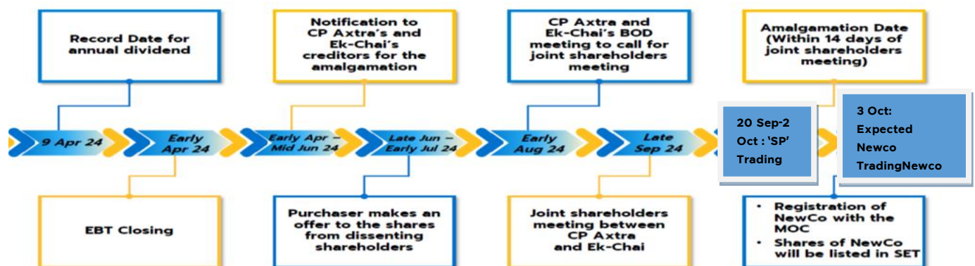
Fig 4. Amalgamation timeline
