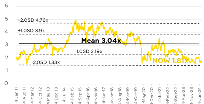
Fig 4. MAJOR's Trailing P/BV
