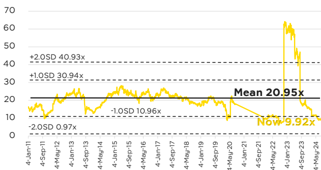
Fig 3. MAJOR's Trailing P/E
