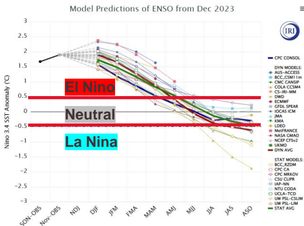
Figure 6: El Nino to transition to neutral conditions in June 2024 and possibly to La Nina in 3Q24
