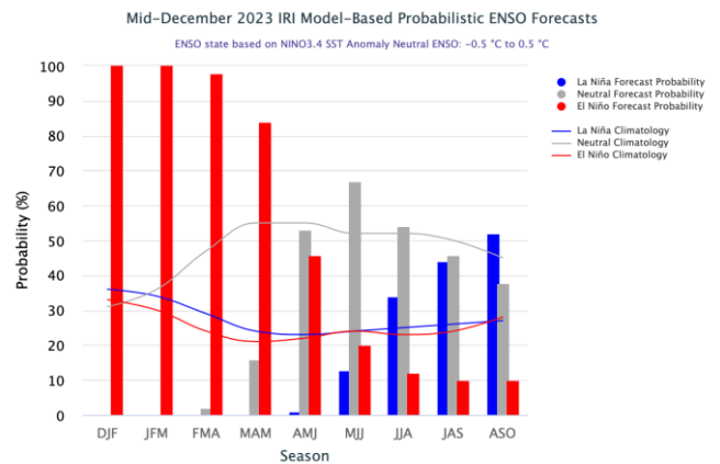
Figure 7: Lower probability of El Nino from June 2024
