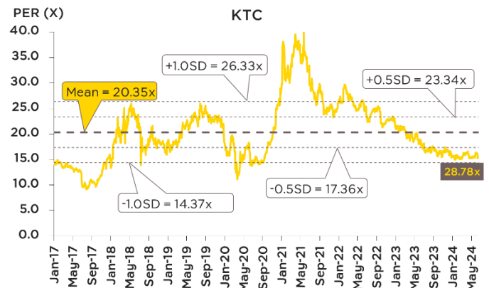
Fig 3. Historical PER band – KTC
