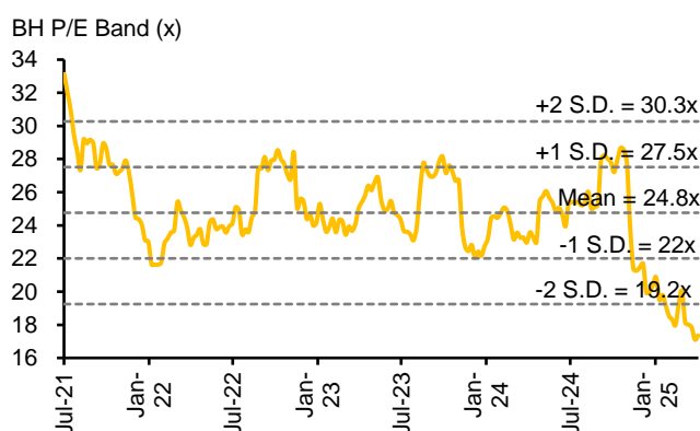
Fig. 4: BH's Prospective P/E band
