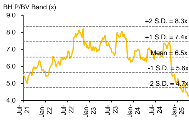
Fig. 5: BH's Prospective P/BV band
