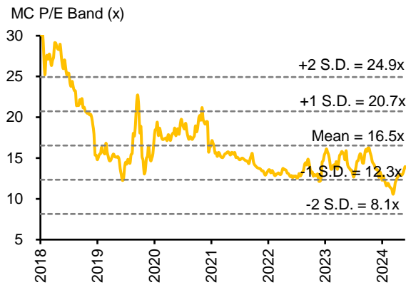
Fig. 2: Forward P/E band
