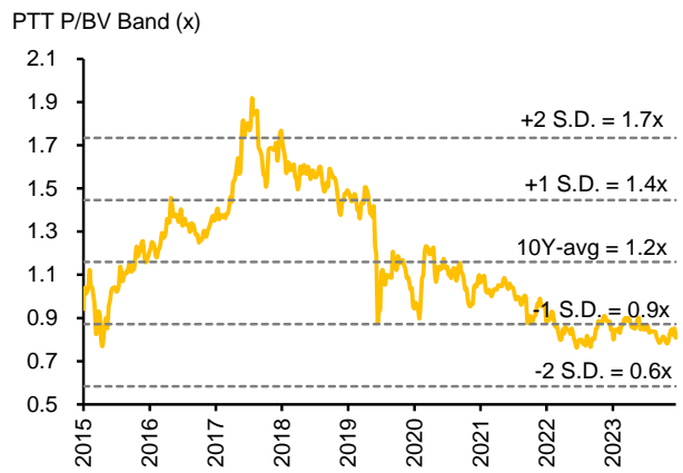
Fig. 6: PBV Band
